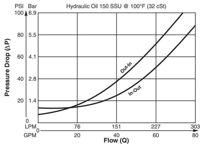
Pressure Drop vs. Flow (Through cartridge only)
