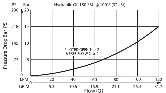
Pressure Drop vs Flow
