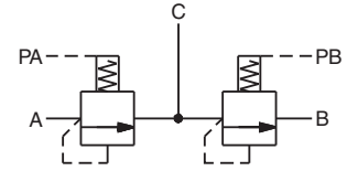
Circuit 3, with LE102A spool logic element.
