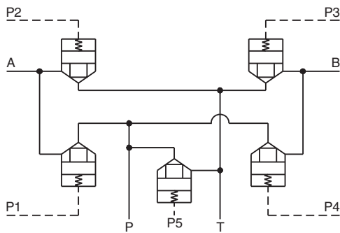
Circuit 1, with LE101A poppet logic elements.
