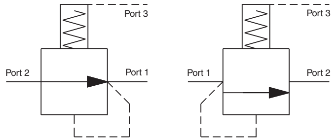
Normally open spool
