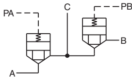
Circuit 1, with LE101A poppet logic element.
