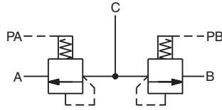
Circuit 2, with LE102A spool logic element.
