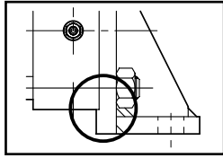
Detail of LC mounting working face (φ32 - φ80)
